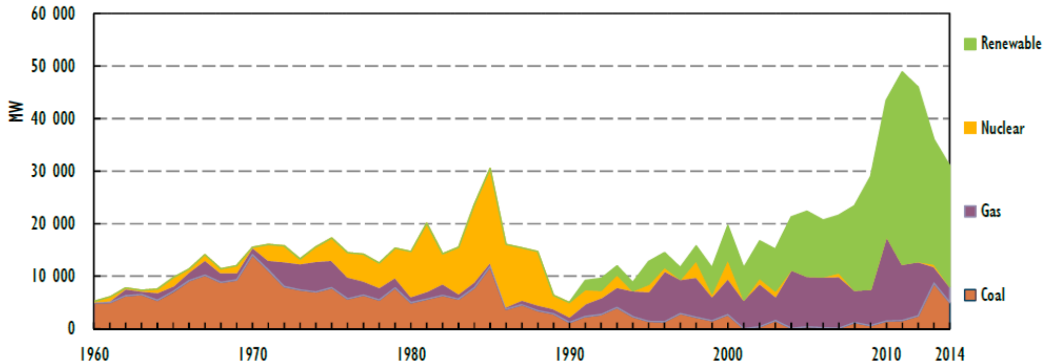
Figure 1.3 • Capacity addition in OECD Europe by technology, 1960-2014
