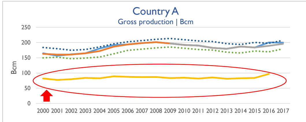
E.g. 01: Model with unbiased sources
