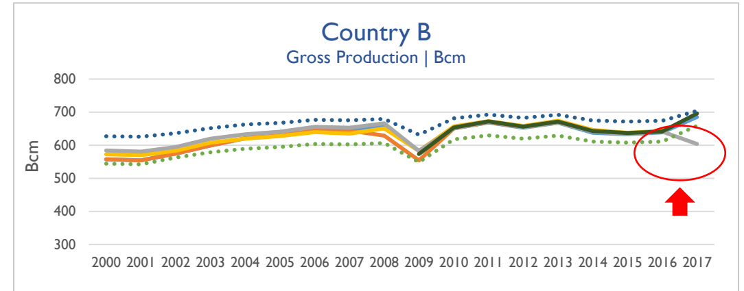
E.g. 02: GECF figures out of the confidence interval
