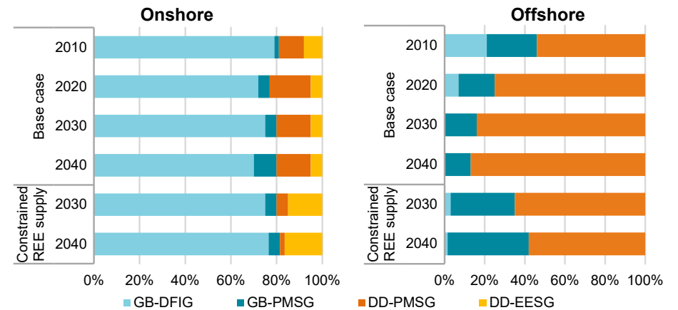
Turbine shares for wind power capacity additions in the SDS
