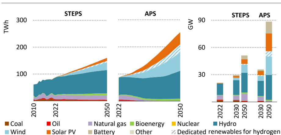
Figure 5.37 ▶ Electricity generation and capacity by fuel and scenario in Colombia
