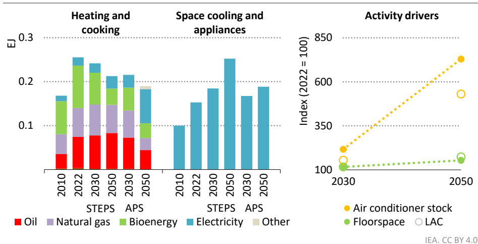
Figure 5.35 ▶ Fuel consumption in buildings by type and scenario in Colombia
