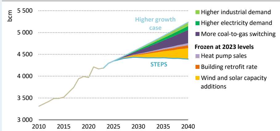
Figure 1.20 ▶ Factors that could lead to continued natural gas demand growth above the levels of the STEPS to 2040
