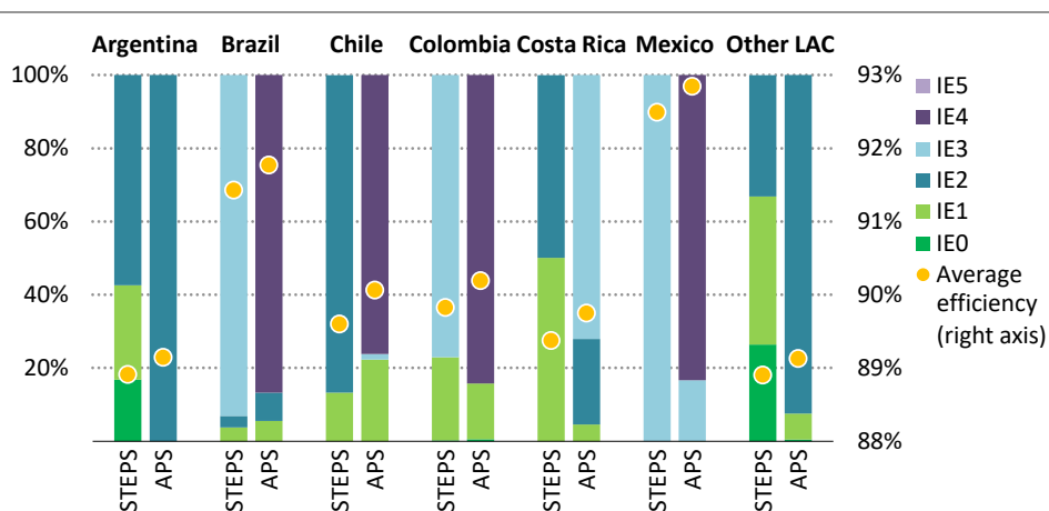
Figure 3.8 ▶ Industrial motor sales by International Efficiency Class and average efficiency in selected countries by scenario, 2030
