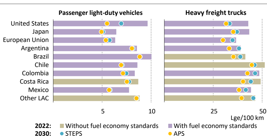
Figure 3.6 ▶ Average fuel consumption of new ICE vehicles in 2022 in selected countries and by scenario in 2030
