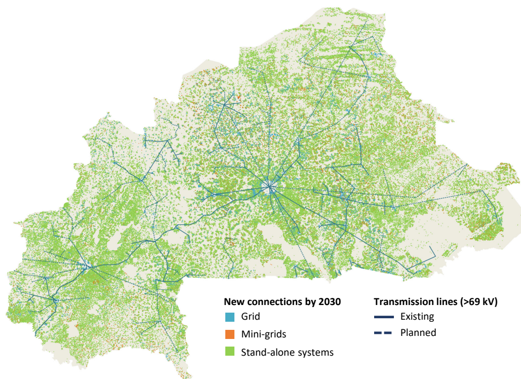
Figure A.1. Electricity access solutions by type in the Africa Case, Burkina Faso
