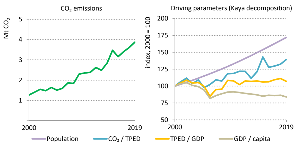
Figure A.8. Energy-related CO 2 emissions and driving parameters, Mauritania
