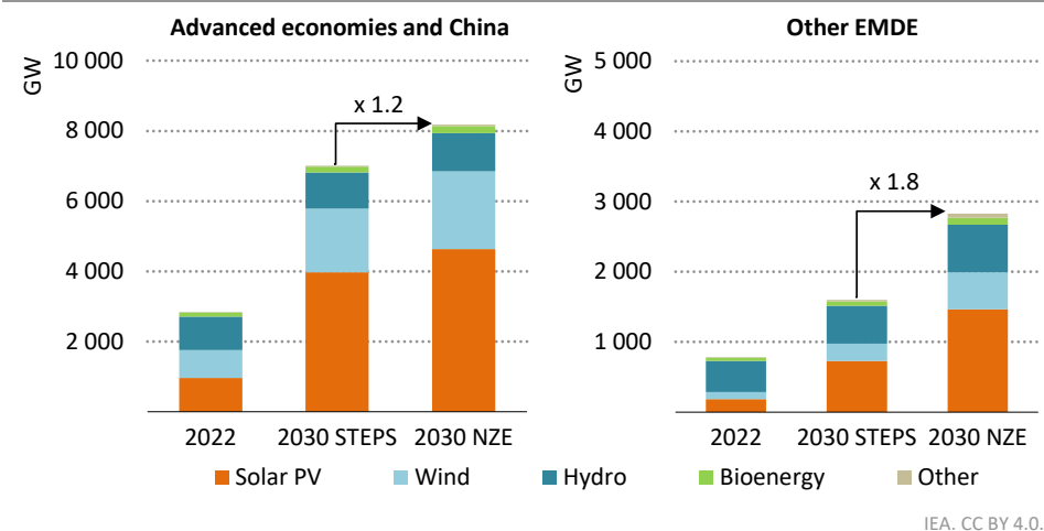
Figure 3.4 ▶ Installed renewables capacity by technology and economic grouping in the STEPS and NZE Scenario, 2022 and 2030
