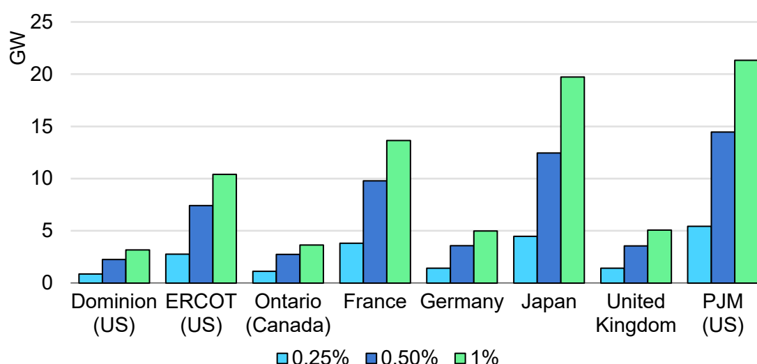
Headroom in selected power systems for different flexibility cases
