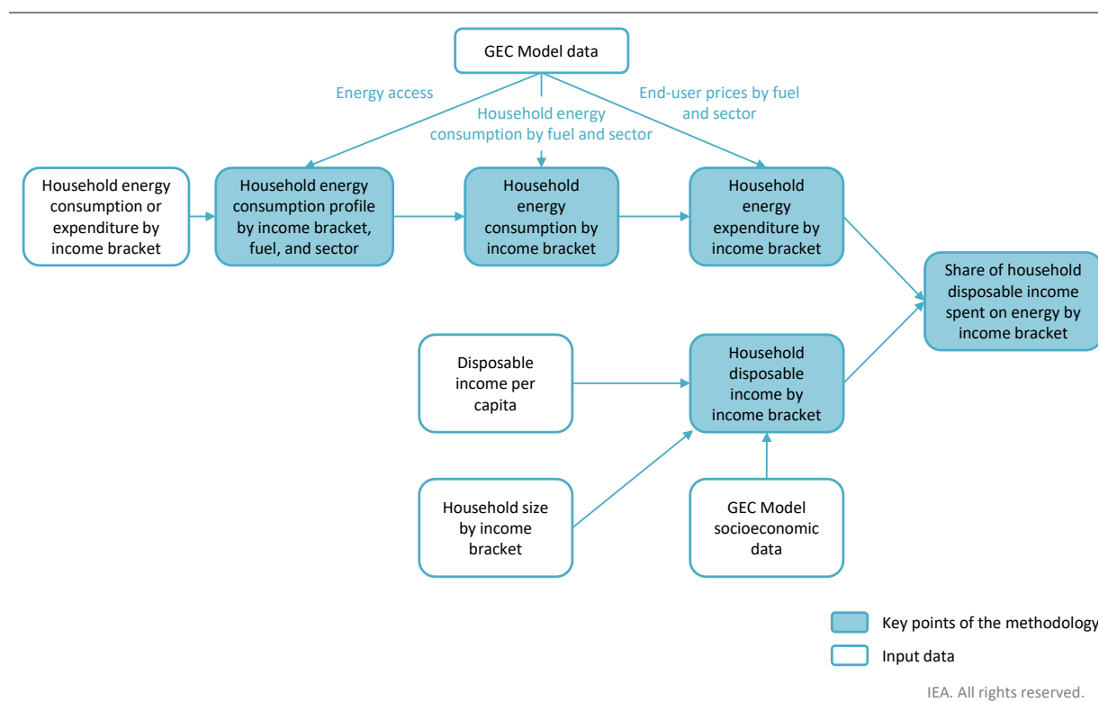
Figure 14.1 ▶ Overview of affordability analysis methodology applied at each GEC Model region level
