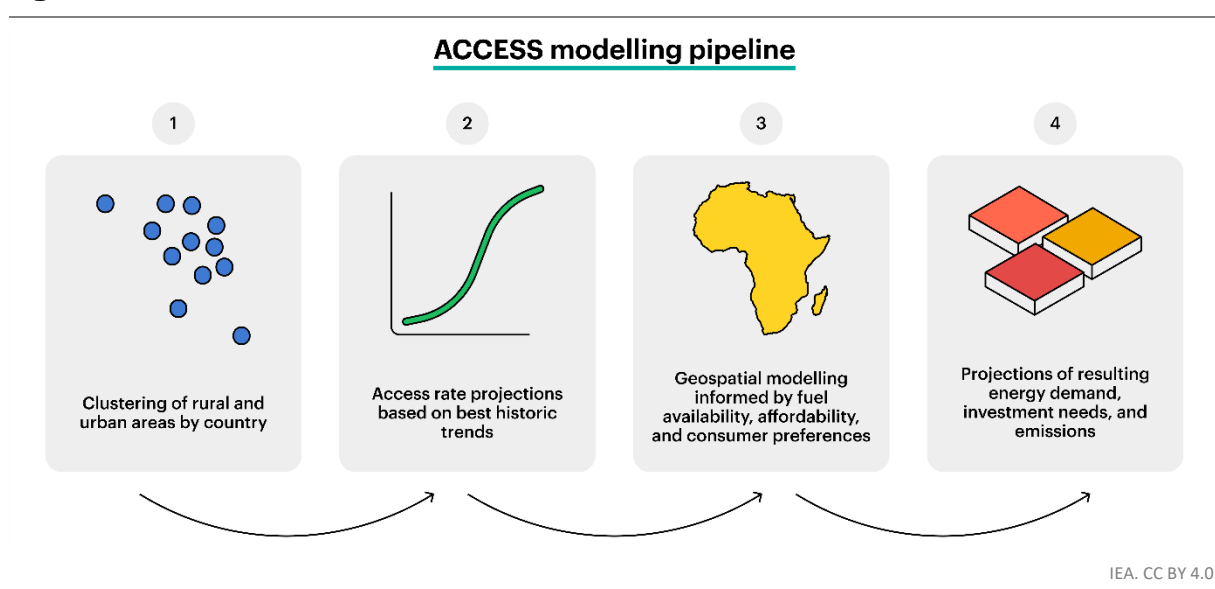
Figure 11.2 ► Modelling framework for the ACCESS
