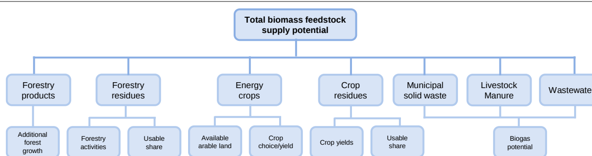
Figure 6.2 ▶ Schematic of biomass supply potentials
