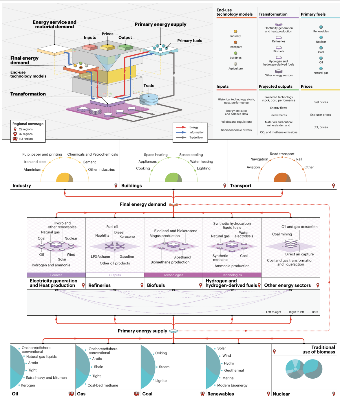
Figure 1.1 ▶ Global Energy and Climate Model overview
