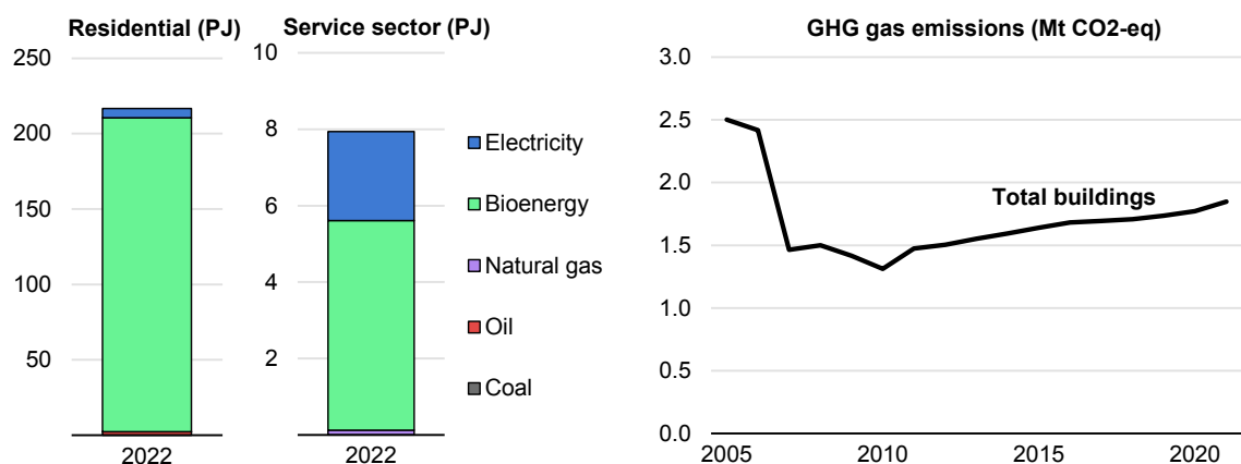
Figure 8.3 Total final energy consumption (2022) and greenhouse gas emissions (2005-2021) from buildings in Mozambique
