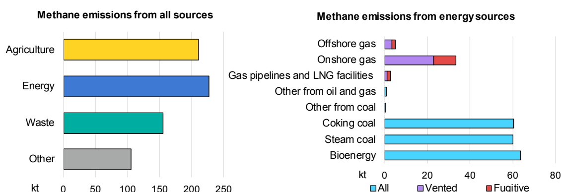
Figure 9.3 Estimates of average cumulative methane emissions by source in Mozambique, 2019-2022
