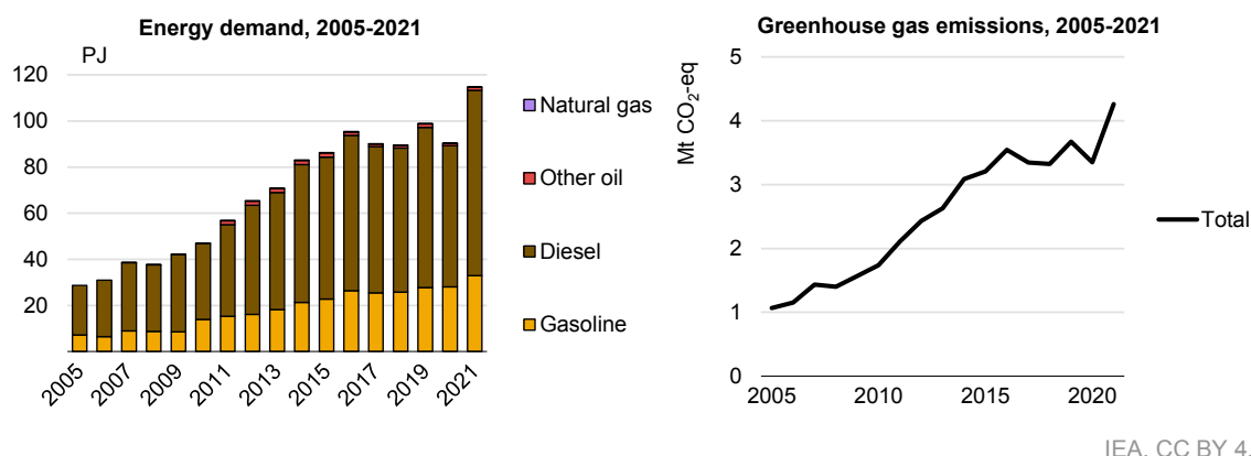
Figure 8.4 Energy demand and emissions in transport by source in Mozambique, 2005-2021
