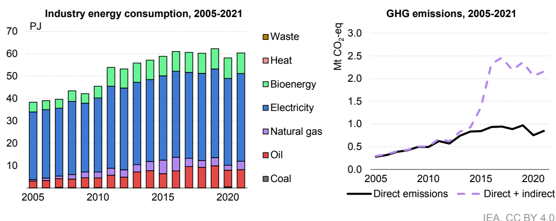
Figure 8.5 Energy demand and emissions in industry by source in Mozambique, 2005-2021
