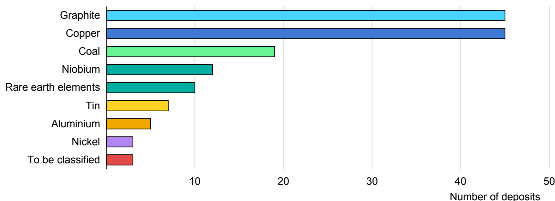
Figure 11.1 Identified mineral deposits of selected commodities in Mozambique, 2024.
