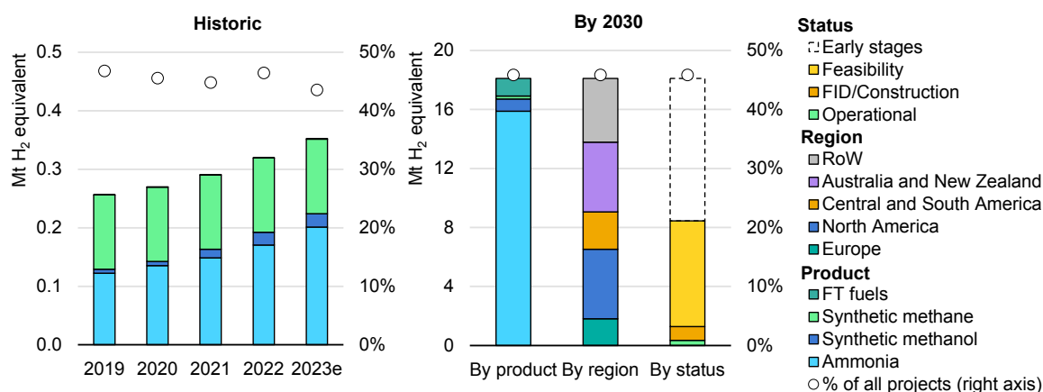
Figure 3.16 Global hydrogen-based fuel production by fuel, region and status, historical and based on announced projects
