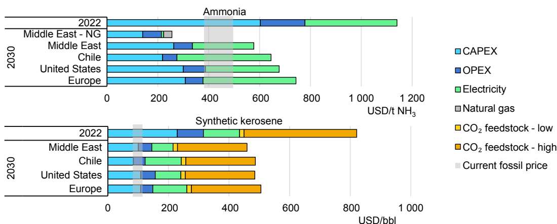
Figure 3.17 Levelised costs of ammonia and synthetic kerosene for electricity-based pathways in 2022 and in the Net Zero Emissions by 2050 Scenario in 2030
