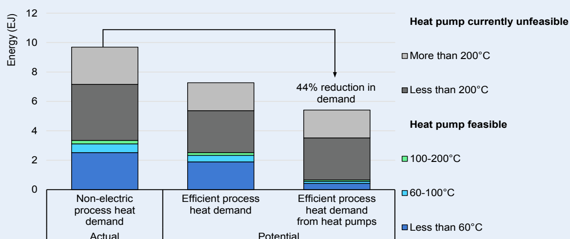
Global non-electric process heat demand in less intensive manufacturing, and estimated efficiency-related savings potential, 2023
