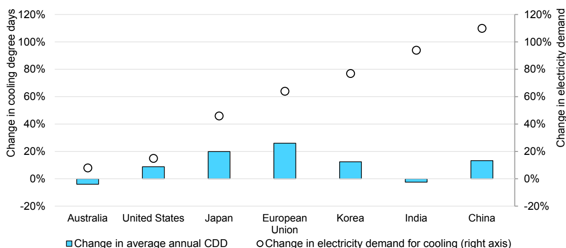
Changes in cooling degree days and electricity demand for cooling between the periods 2010-2019 and 2020-2024
