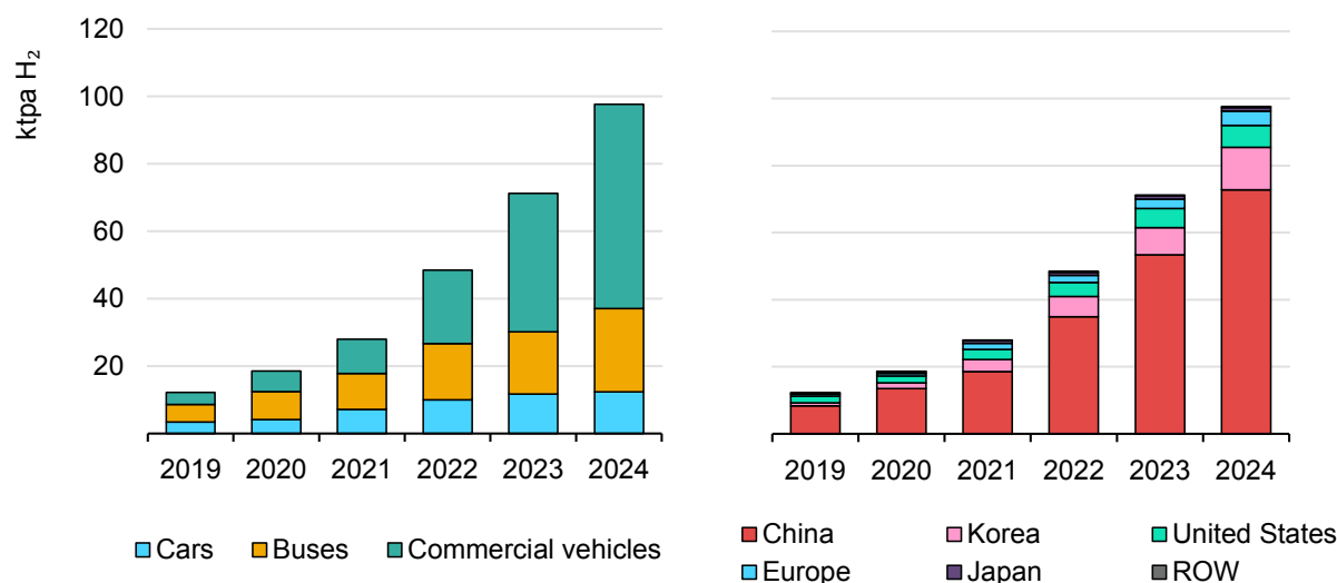
Figure 2.10 Hydrogen demand in road transport by vehicle mode and region, 2019-2024
