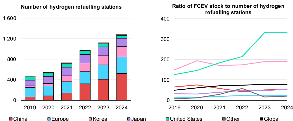
Figure 2.13 Number of hydrogen refuelling stations by region and ratio of fuel cell electric vehicle stock to number of stations, 2019-2024
