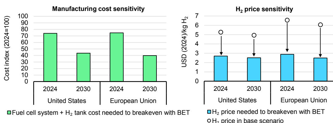
Figure 2.15 Breakeven hydrogen price, fuel cell system and hydrogen tank manufacturing costs needed to reach total cost of ownership parity with battery electric trucks in selected regions, 2024-2030
