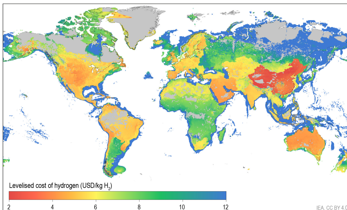
Figure 3.9 Hydrogen production cost from electrolysis using hybrid solar PV and onshore wind, and from offshore wind, in the Stated Policies Scenario, 2030
