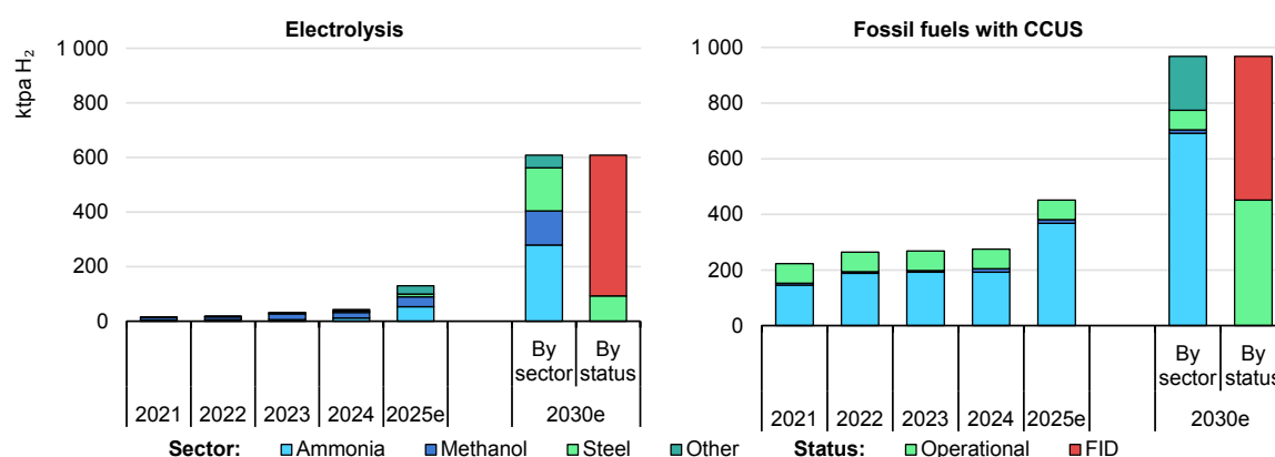
Figure 2.8 Onsite production of low-emissions hydrogen for industry applications by sector and by status, 2021-2030
