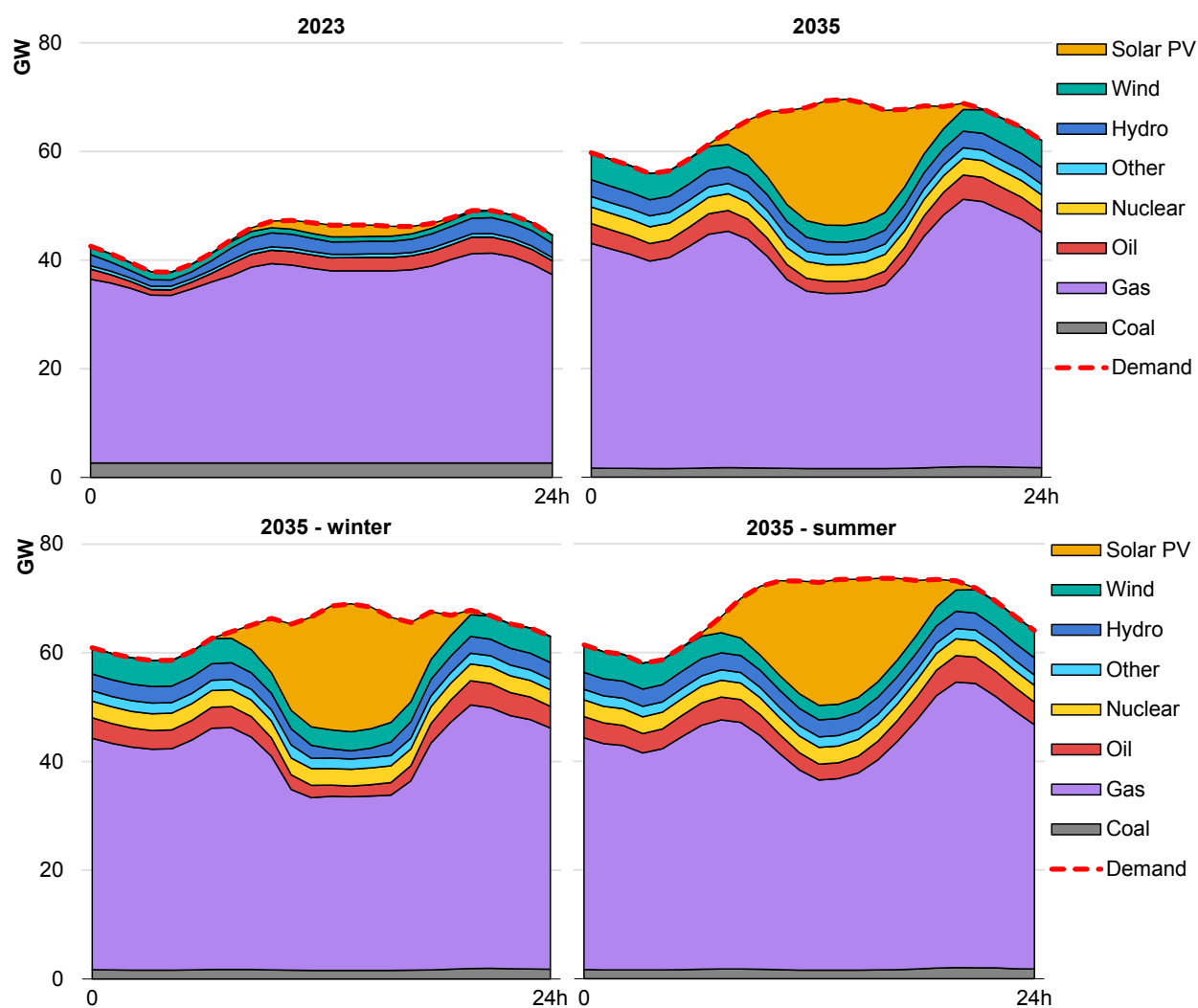
Figure 3.3 Average daily electricity supply by source in North Africa in the Stated Policies Scenario, 2023 and 2035
