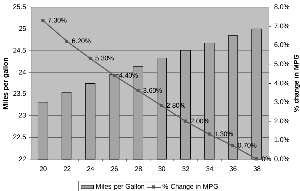
Figure 5.1. Fuel Economy versus Inflation Pressure (38 to 20 PSI)
