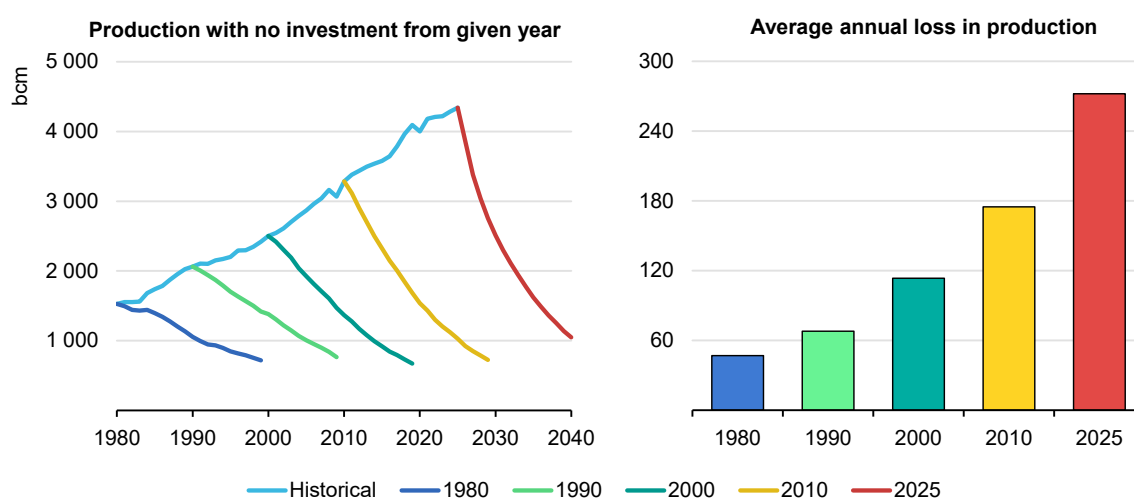
Figure 39 Natural gas production under natural decline rates worldwide
