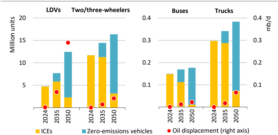
Figure 2.9 ▶ Electrification share of transport stock and oil displacement in Colombia in the APS, 2024-2050
