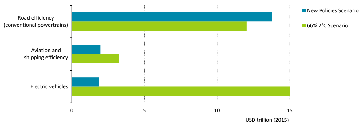
Figure 2.30 • Global cumulative transport investment in the New Policies and 66% 2°C Scenarios, 2016-50
