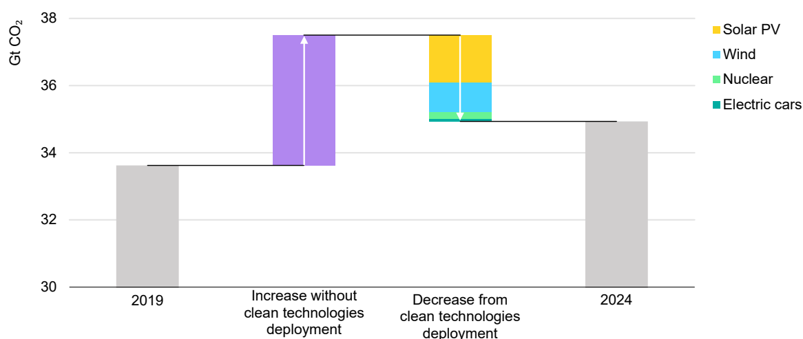
Change in CO 2 emissions from fuel combustion and avoided emissions from deployment of selected clean technologies, 2019-2024
