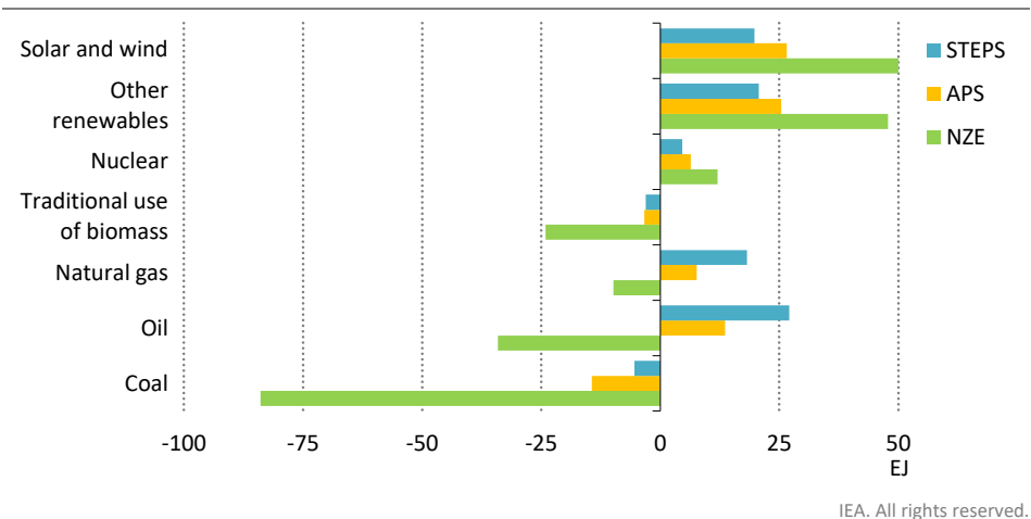
Figure 4.12 ▶ Change in global total energy supply by fuel and scenario, 2020-2030
