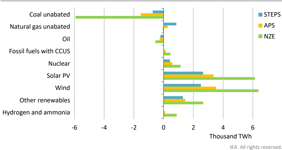
Figure 4.23 ▶ Change in electricity generation by source and scenario, 2020 to 2030
