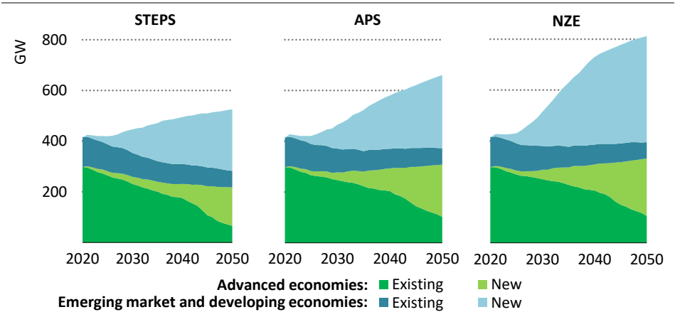
Figure 4.24 ▶ Nuclear power capacity by scenario, 2020-2050
