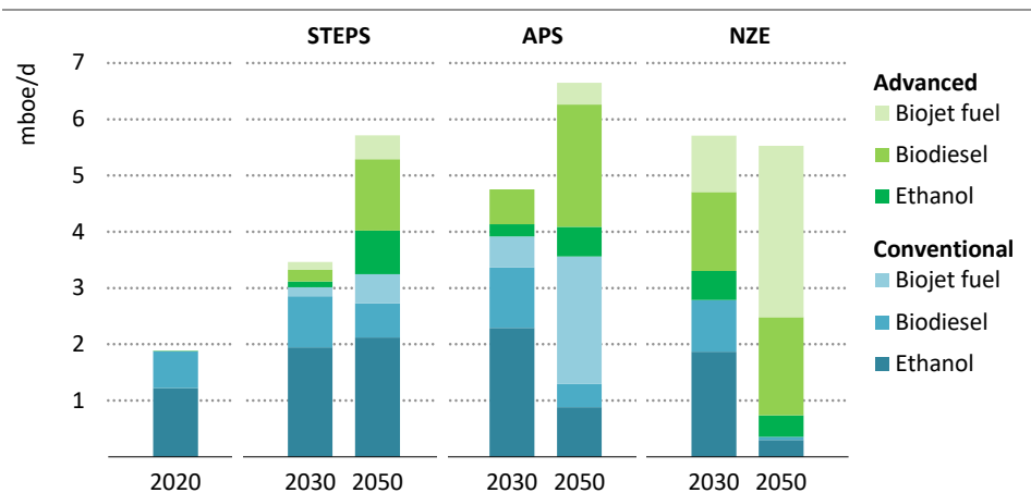
Figure 5.10 ▶ Liquid biofuel demand by type and scenario
