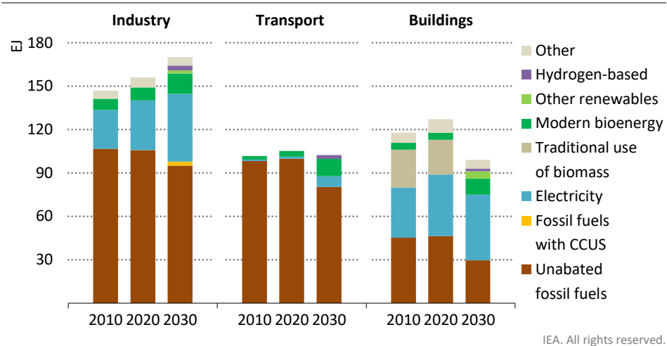
Figure 3.3 ▶ Final energy consumption by source and sector to 2030 in the Net Zero Emissions by 2050 Scenario
