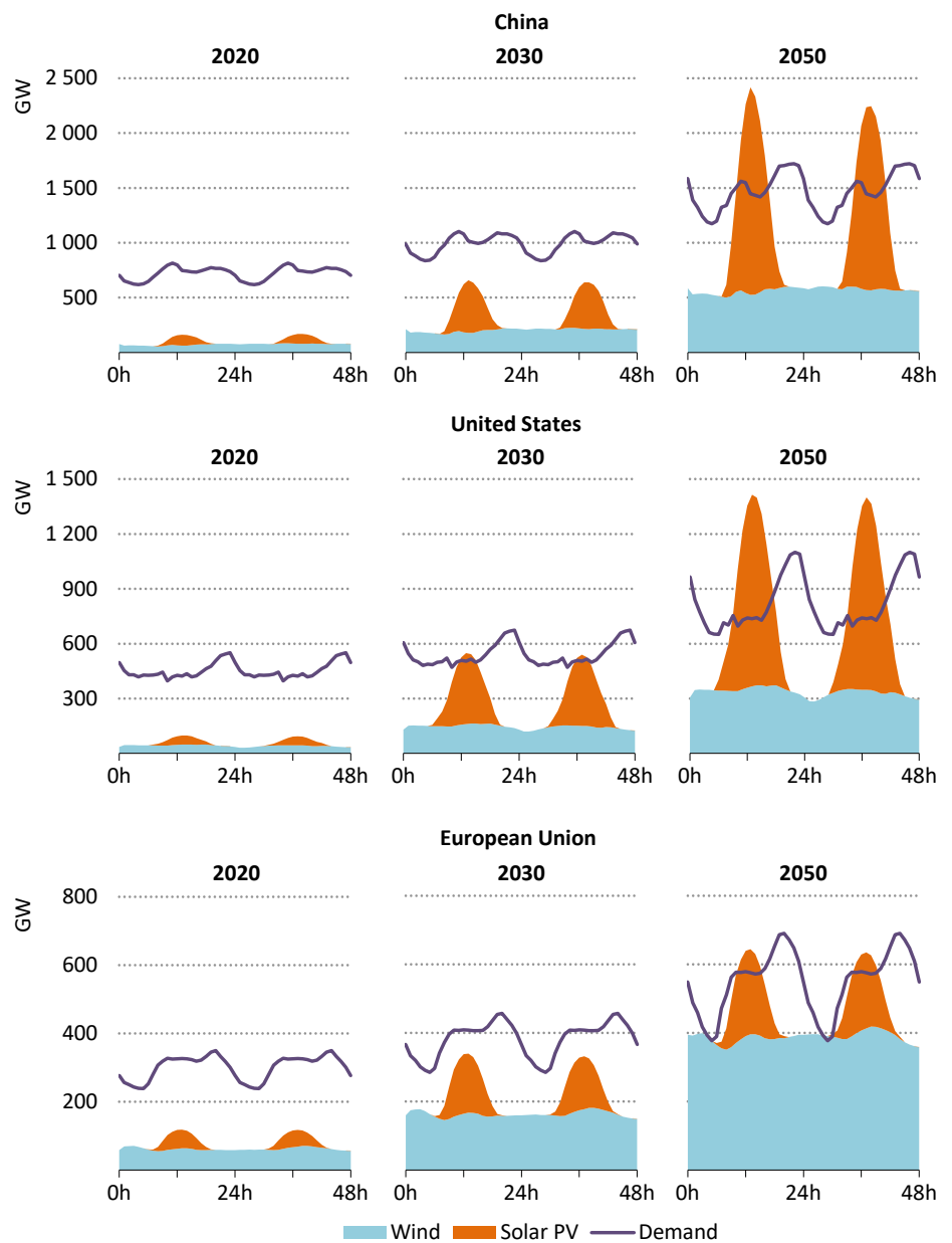
Figure 6.4 ▶ Wind and solar PV generation and electricity demand for sample days in Q1 by region in the Announced Pledges Scenario
