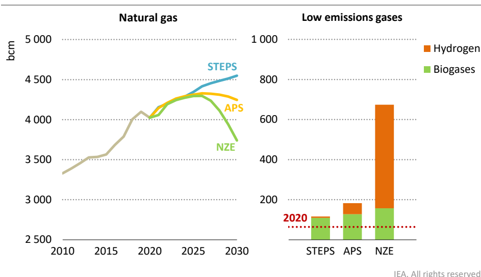
Figure 5.12 ▶ Natural gas use over time and low emissions gas supply in 2030
