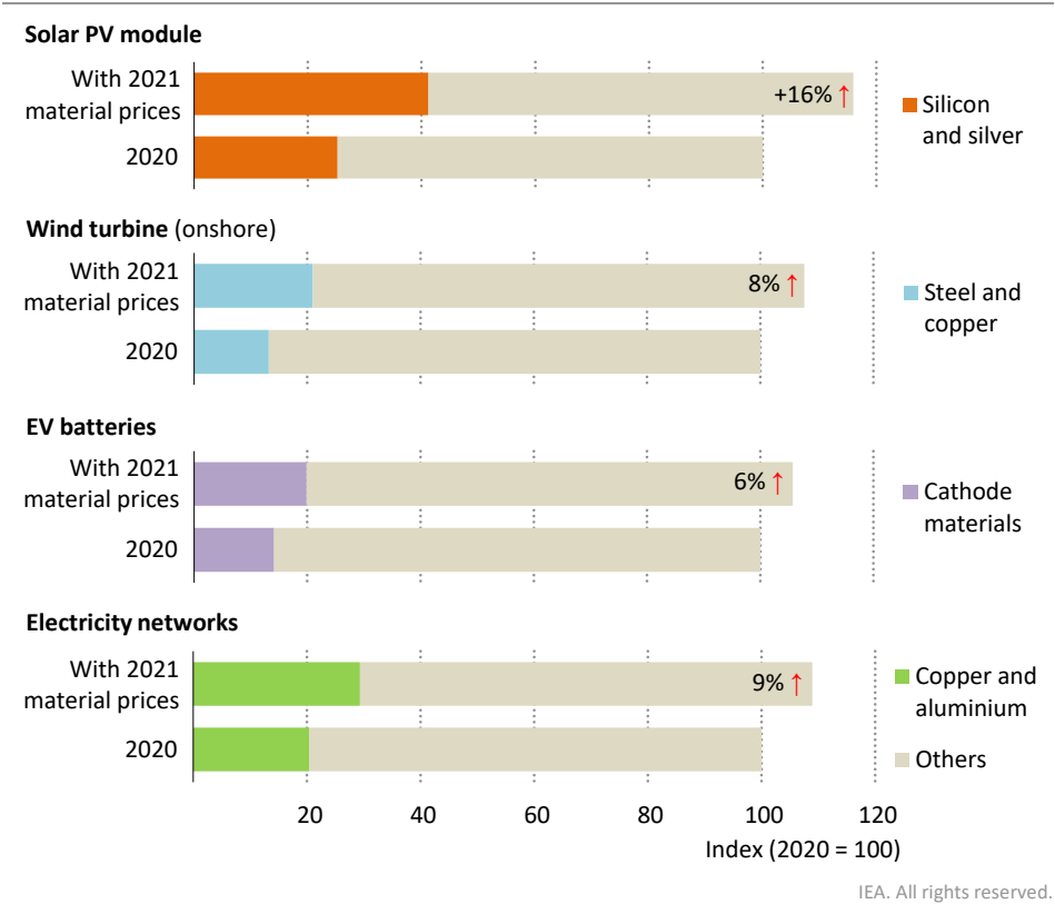
Figure 6.17 ▶ Impacts of 2021 material price increases on the costs of selected clean energy technologies
