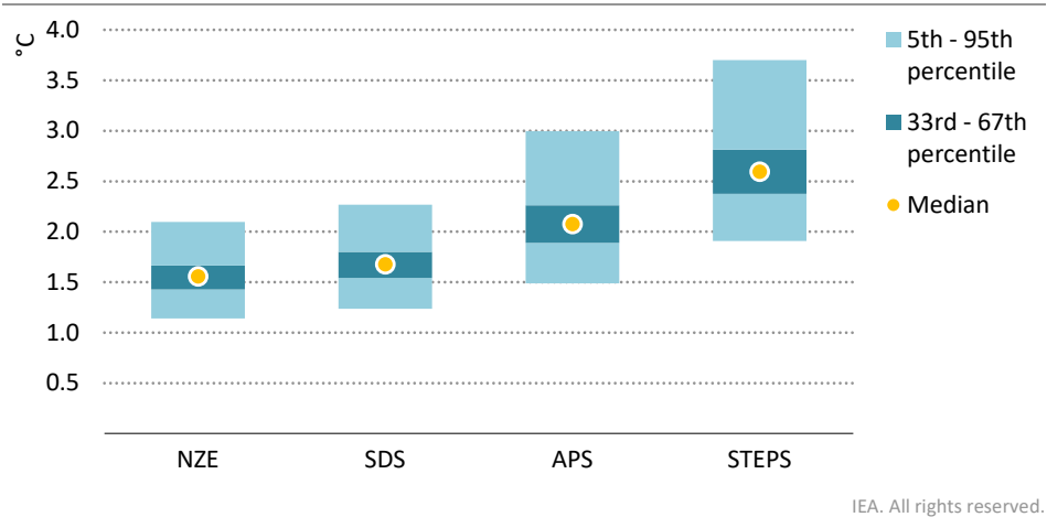
Figure 1.6 ▶ Peak temperature rise in the WEO-2021 scenarios
