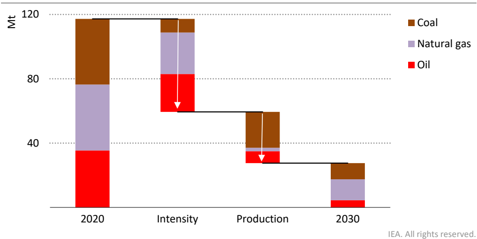
Figure 1.9 ▶ Methane emissions from fossil fuel operations and reductions to 2030 in the Net Zero Emissions by 2050 Scenario
