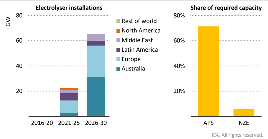
Figure 5.19 ▶ Planned and announced electrolyser installations to 2030 and their proportion of required additions, 2021-2030
