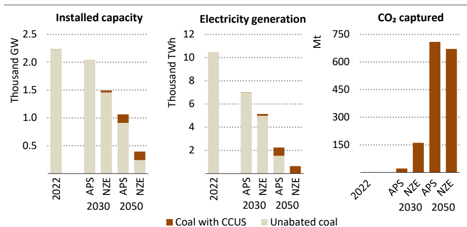
Figure 2.7 ▶ Global coal-fired power generating capacity, output and CO 2 capture by scenario
