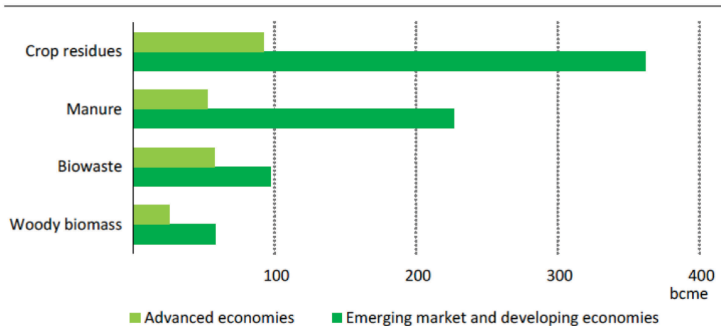
Figure 2.2 ▶ Potential for biogases by feedstock
