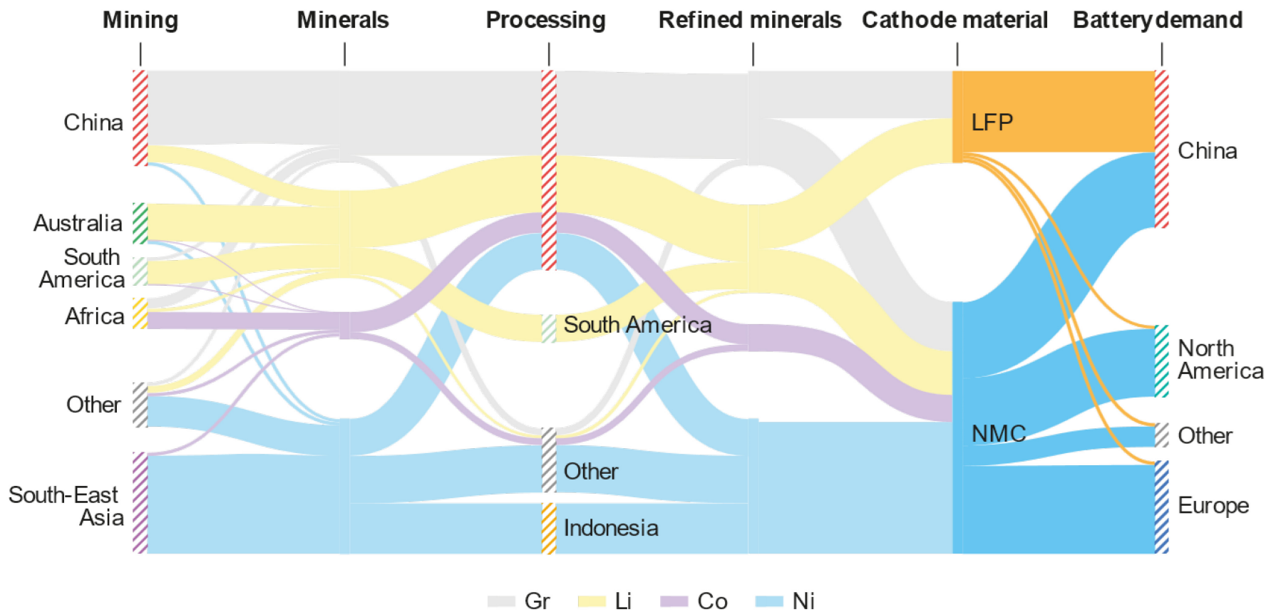
Electric vehicle battery minerals’ supply chain from extraction to end-use, by mineral value, 2023
