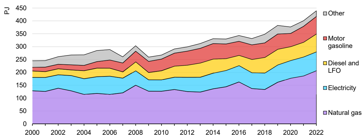
Total final energy consumption by energy source in Azerbaijan, 2000-2022
