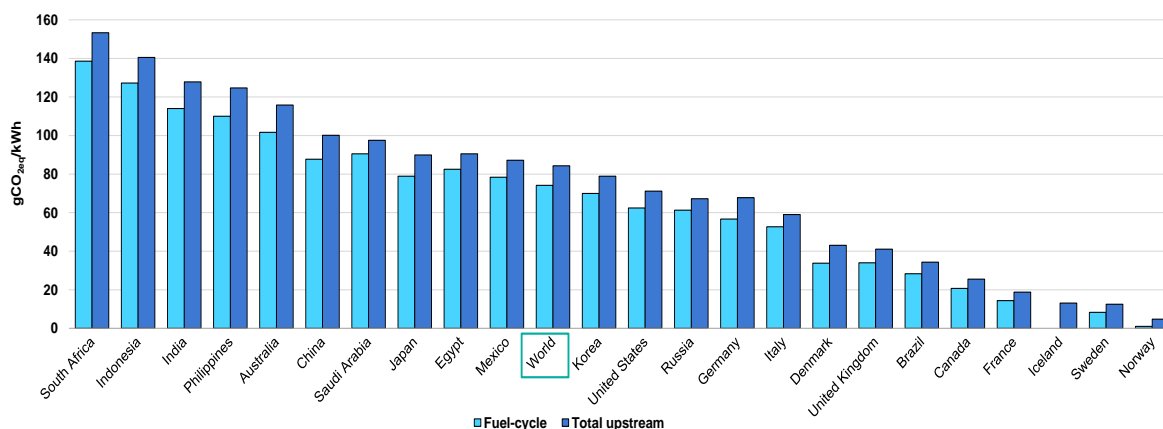
Fuel-cycle vs Total upstream emission factors - selected economies - year 2021
