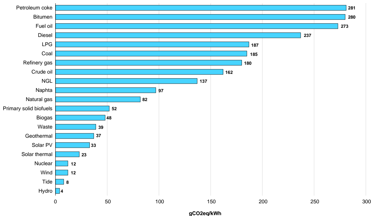
Total upstream electricity generation emission factors - global central tendencies - year 2021
