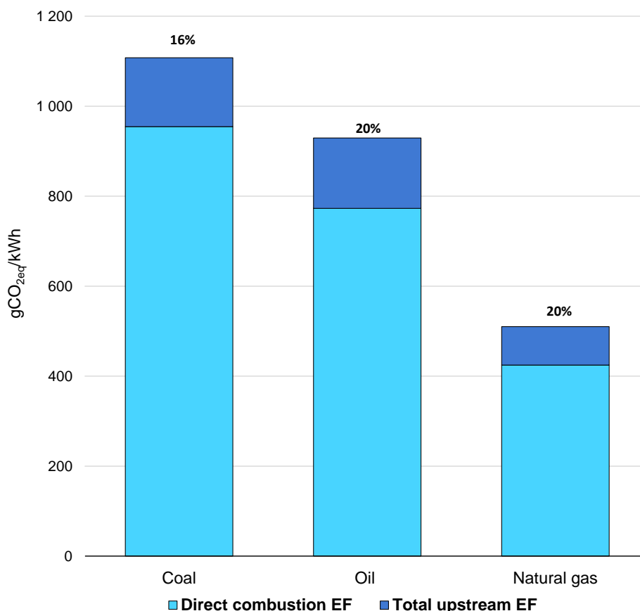
Contribution of direct vs upstream emission factor in electricity generation GHG intensity per fuel - World* - year 2021
