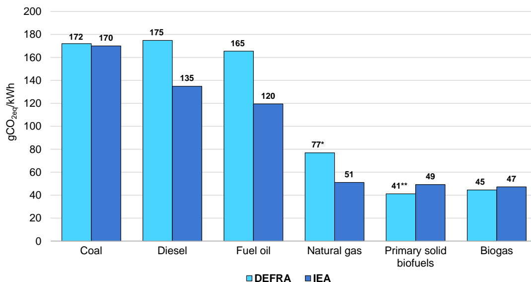
Fuel-cycle emission factors comparison - UK - year 2021
