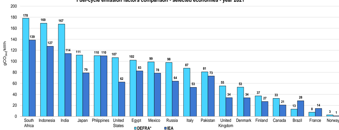
Fuel-cycle emission factors comparison - selected economies - year 2021
