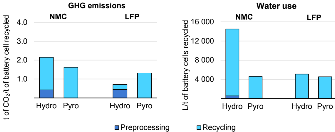
Figure 3.9 GHG emissions and water use for NMC and LFP recycling processes
