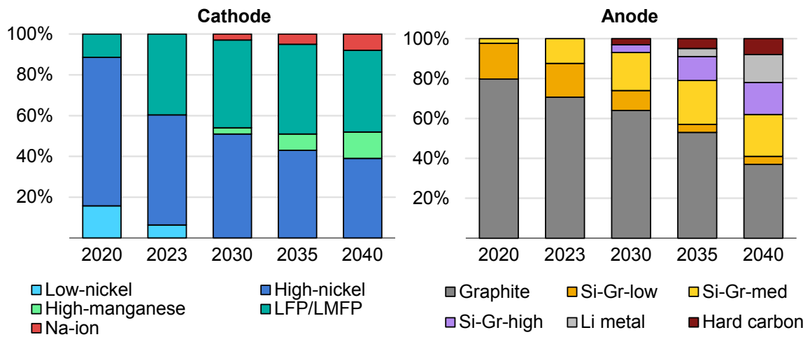
Figure 2.8 Electric car battery cathode and anode chemistry development projections, base case, 2020-2050
