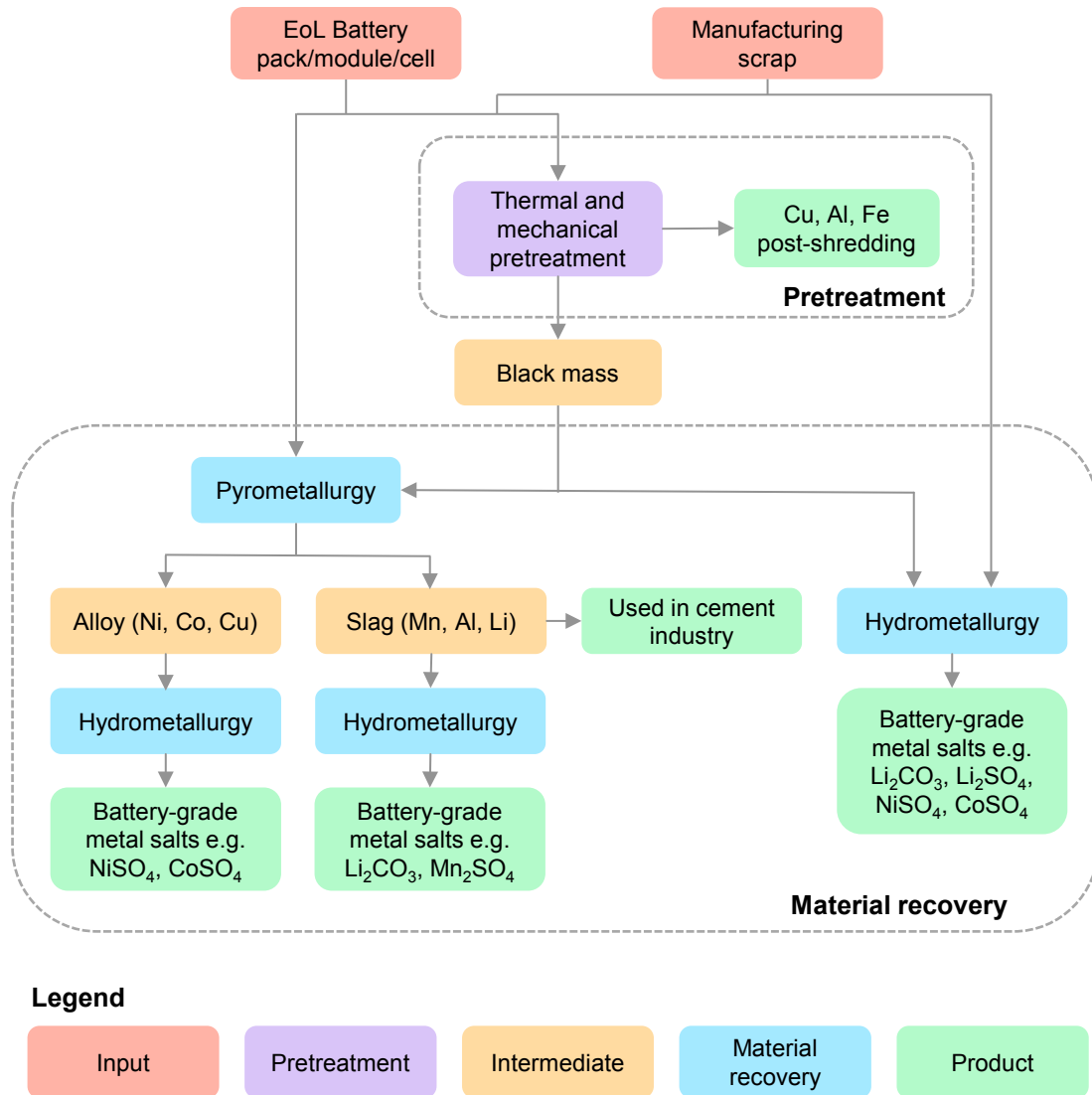
Figure 2.4 Battery recycling processes and pathways
