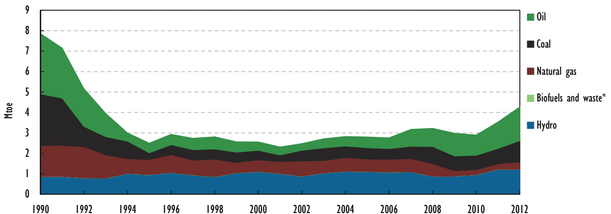
Figure 6.1.2 TPES, Kyrgyzstan, 1990-2012
