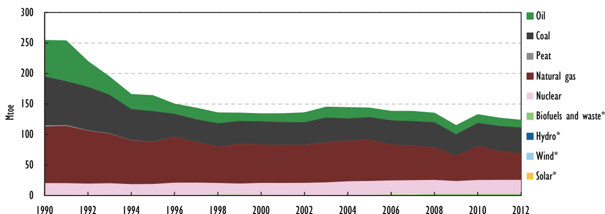
Figure 10.1.3 TPES, Ukraine, 1990-2012
