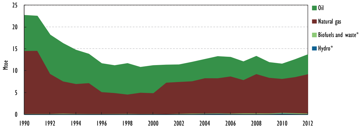
Figure 2.1.3 TPES, Azerbaijan, 1990-2012
