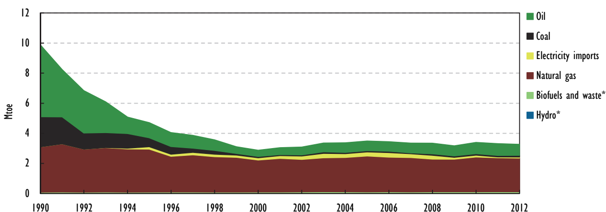
Figure 7.1.2 TPES, Moldova, 1990-2012
