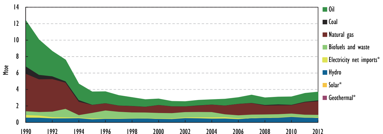
Figure 4.1.2 TPES, Georgia, 1990-2012
