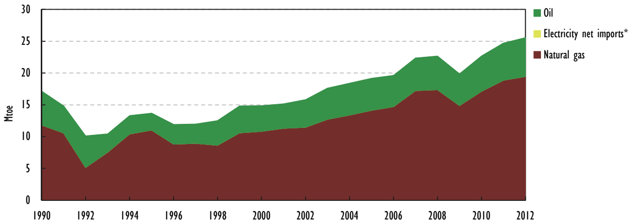
Figure 9.1.3 TPES, Turkmenistan, 1990-2012
