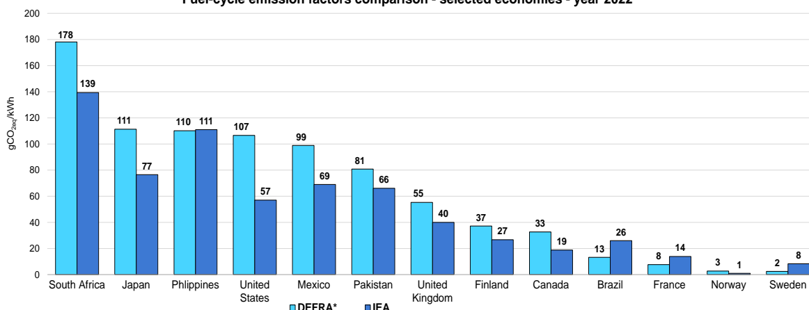
Fuel-cycle emission factors comparison - selected economies - year 2022
