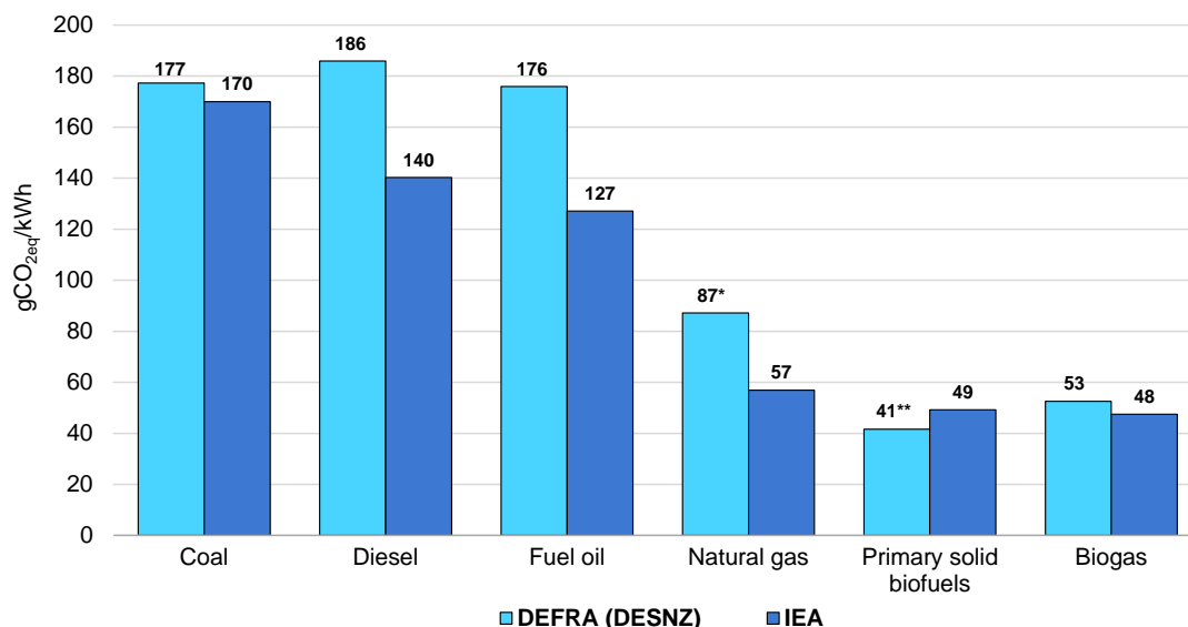
Fuel-cycle emission factors comparison - UK - year 2022
