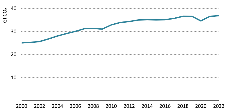
Figure 1.1 ▶ Global energy sector CO 2 emissions, 2000-2022
