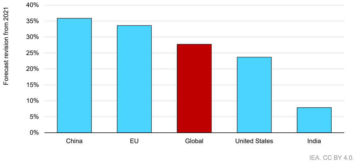
Figure 1.1 Upward revisions to renewable capacity expansion forecasts from Renewables 2021 to Renewables 2022
