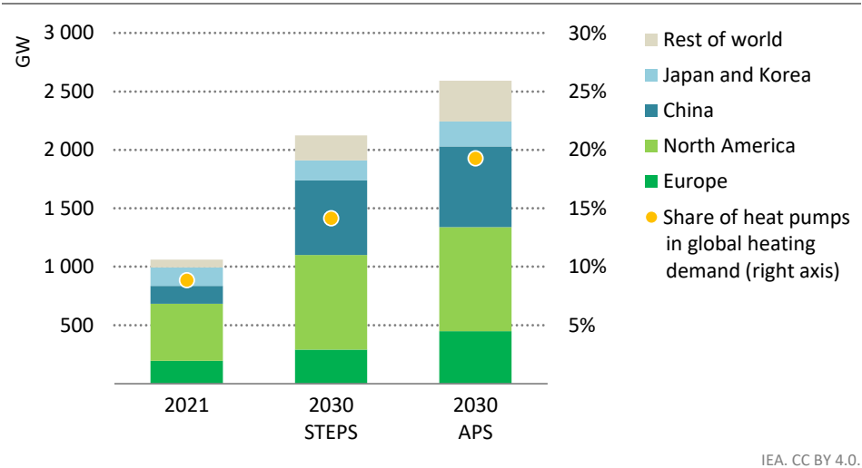
Figure 1.7 ▶ Heat pump capacity in buildings by country/region and scenario, 2021 and 2030
