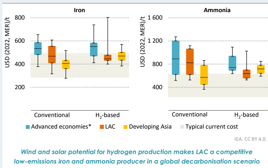
Figure 4.14 ▶ Levelised cost of production of iron and ammonia by process type in selected regions in the NZE Scenario, 2030
