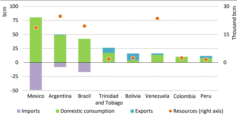
Figure 3.26 ▶ Natural gas demand, imports, exports and resources in selected countries, 2021
