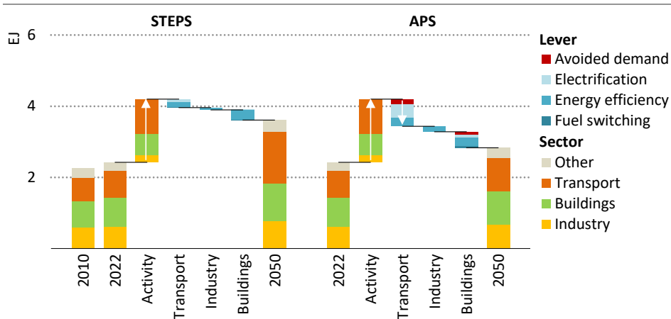
Figure 5.8 ▶ Final energy consumption by scenario in Argentina
