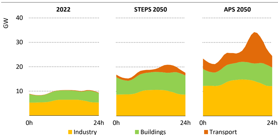
Figure 5.28 ▶ Average electricity daily load profile by scenario in Chile
