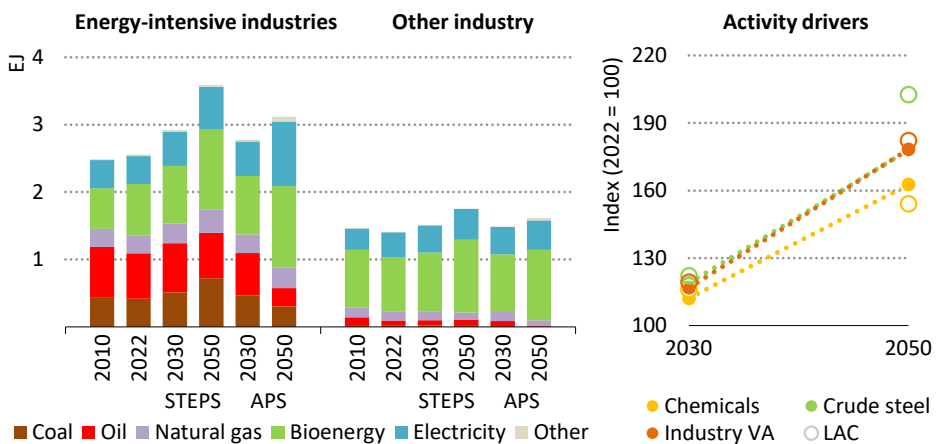
Figure 5.17 ▷ Fuel consumption in industry by type and scenario in Brazil
