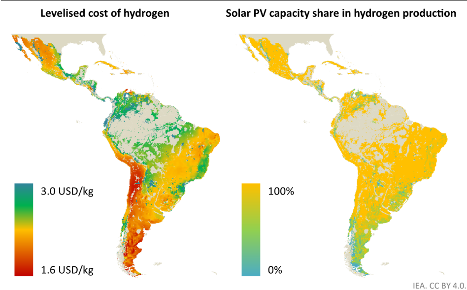
Figure 3.15 ▶ Levelised hydrogen production costs and share of solar PV from hybrid solar PV and wind systems in LAC, 2030
