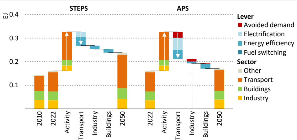
Figure 5.40 ▾ Final energy consumption by scenario in Costa Rica
