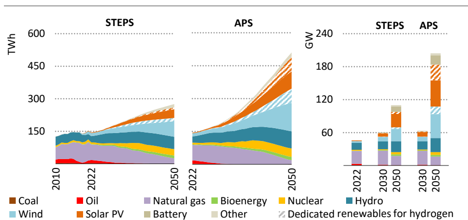
Figure 5.13 ▶ Electricity generation and capacity by fuel and scenario in Argentina
