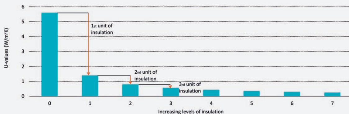
Figure 3.9 Representation of insulation performance with diminishing returns
