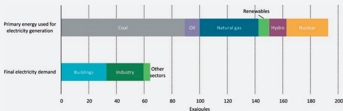
Figure 1.5 Energy use for power generation and total final electricity demand, 2010
