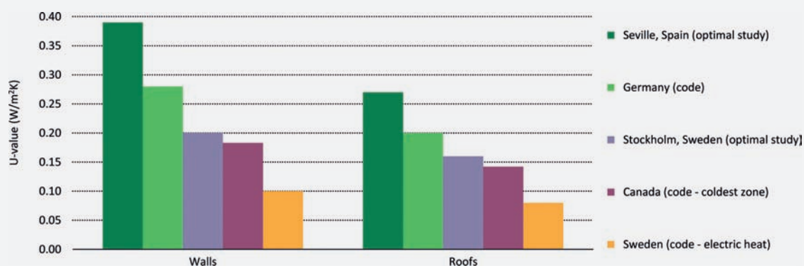
Figure 3.10 Wall and roof U-value comparisons for reference perspectives
