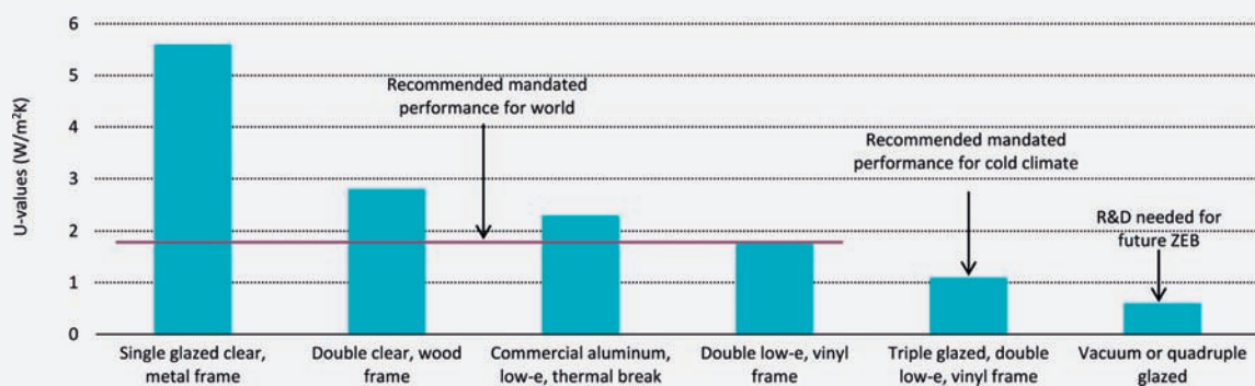
Figure 3.7 Typical window U-values for common products in the market place
