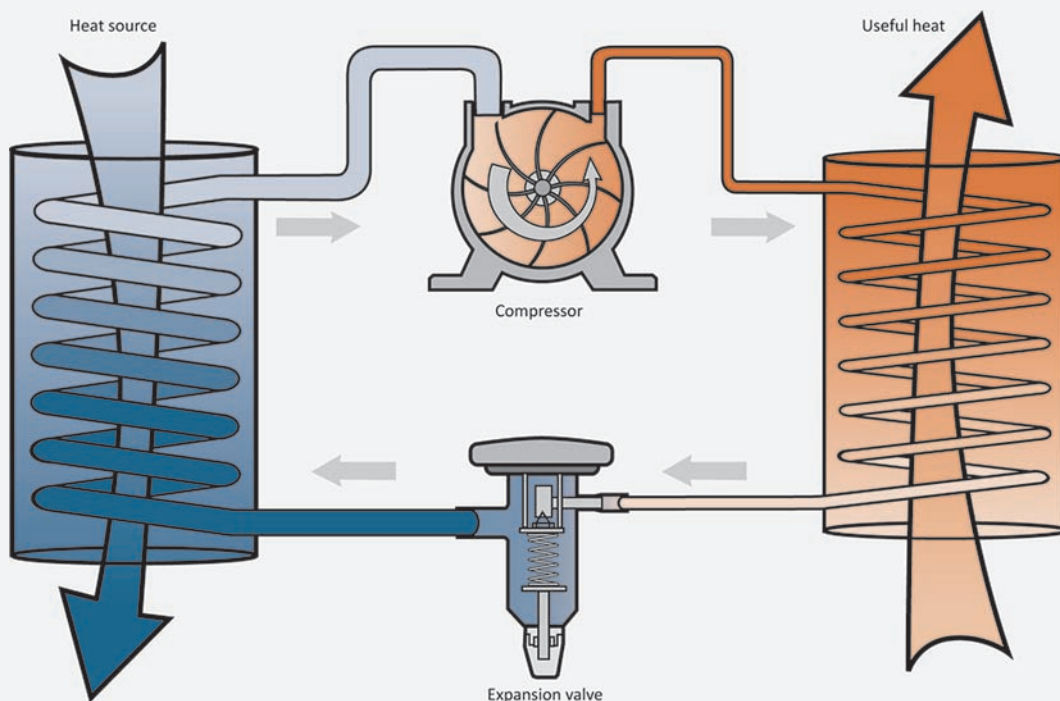
Figure 4.6 Basic concept of a heat pump
