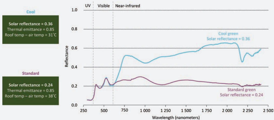
Figure 3.12 Cool-coloured material and performance
