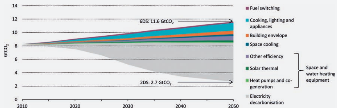
Figure ES.1 Contribution of CO 2 emissions reduction in the buildings sector
