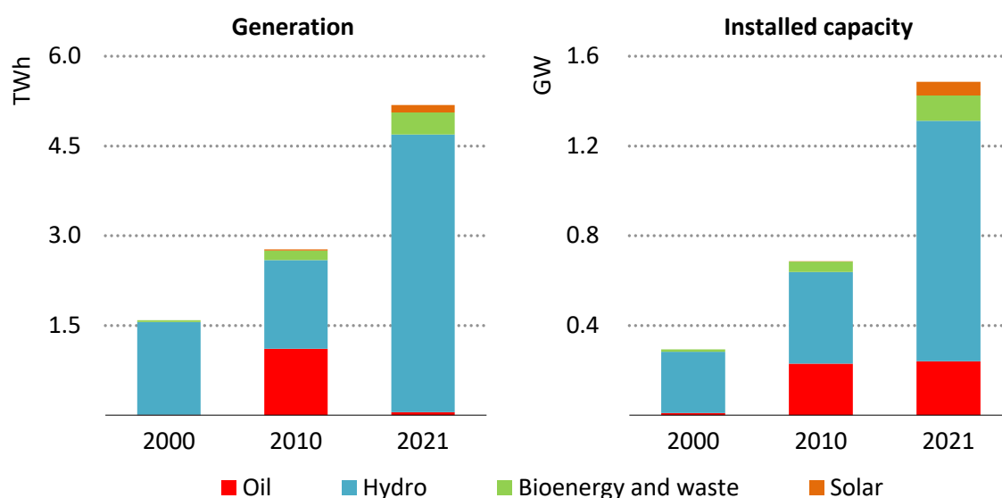
Figure 1.4 Power generation and installed capacity in Uganda, 2000-2021
