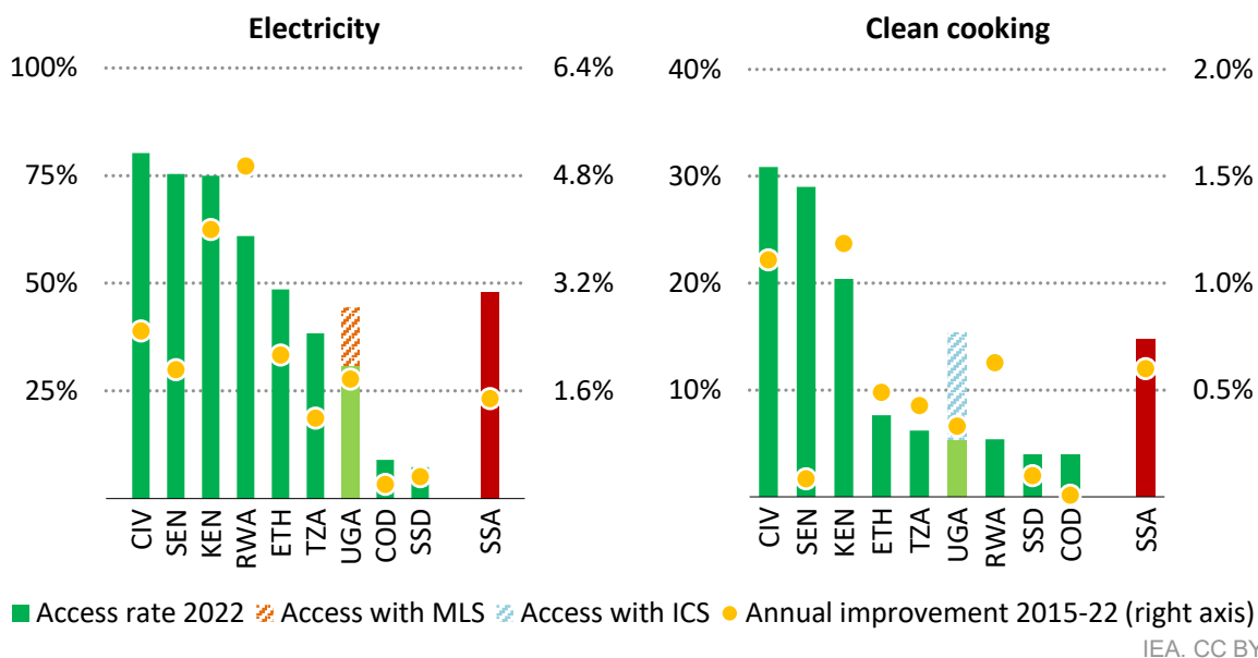
Figure 1.3 Electricity and clean cooking access rates in Uganda, 2022
