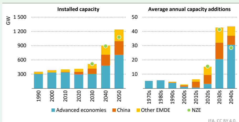
Figure 7.14 ► Global nuclear installed capacity and capacity additions to reach the tripling target by 2050 relative to the NZE Scenario
