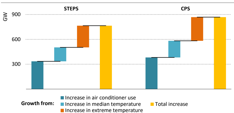
Figure 5.24 ▶ Aggregated peak electricity demand growth related to cooling and impact of extreme heat by scenario, 2035
