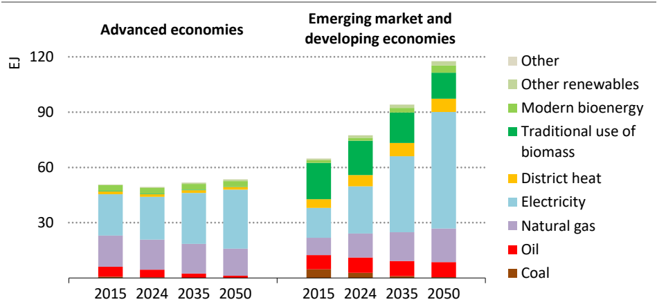
Figure 3.9 ▶ Energy demand in buildings by economic grouping and fuel in the CPS to 2050
