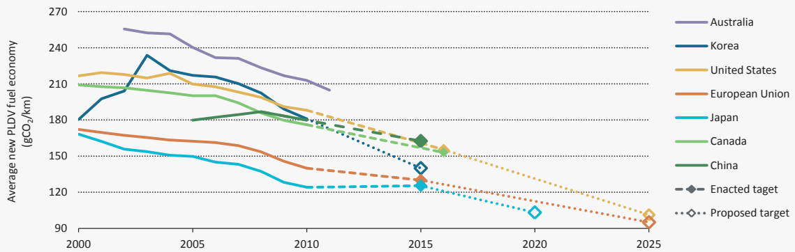
Figure 1.26 Vehicle fuel economy, enacted and proposed standards
