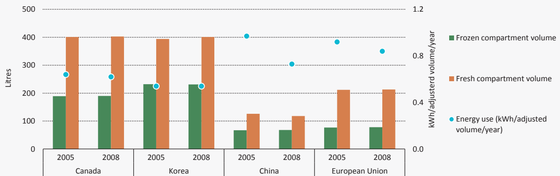
Figure 1.24 Energy use and volume for combined refrigerator and freezer units
