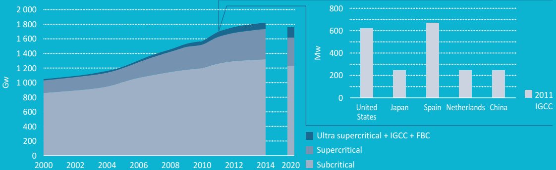
1.6: Coal technology deployment by technology (2000-14) and ETP 2DS
