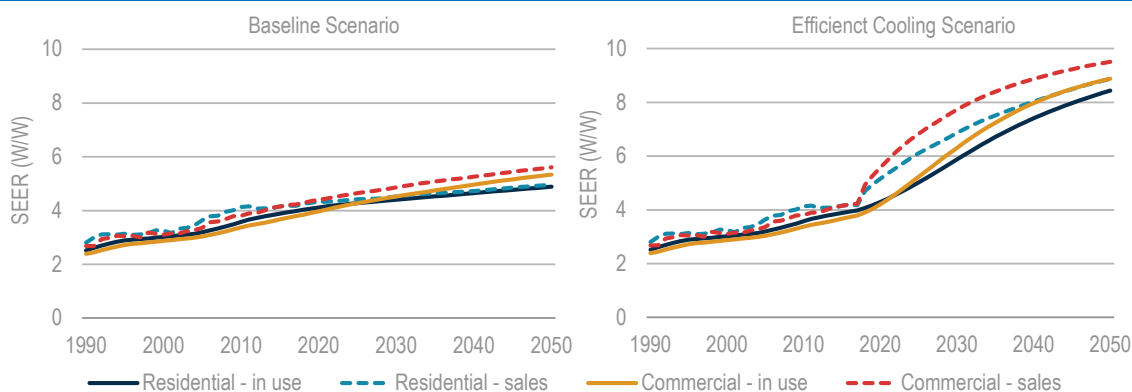
Figure 3.15 • Average global SEER of ACs by scenario
