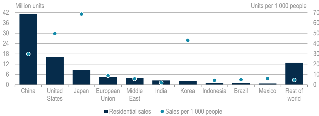
Figure 1.5 • Sales of residential ACs by country/region, 2016
